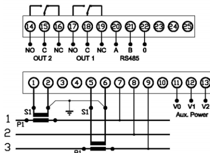
Circuito trifase a 3 fili (2 TA, inserz. ARON) Three-phase 3 wires circuit (2 CT, ARON)
